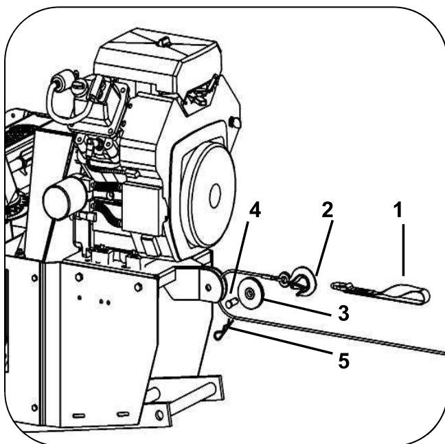
Lift system
