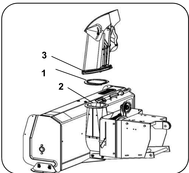
Chute installation
