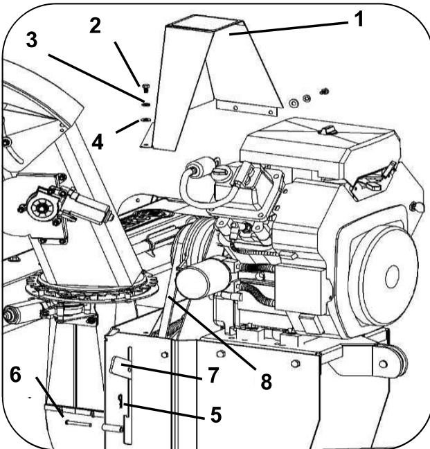
Belt replacement
