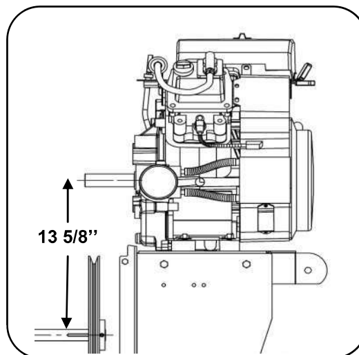
Height of the engine shaft
