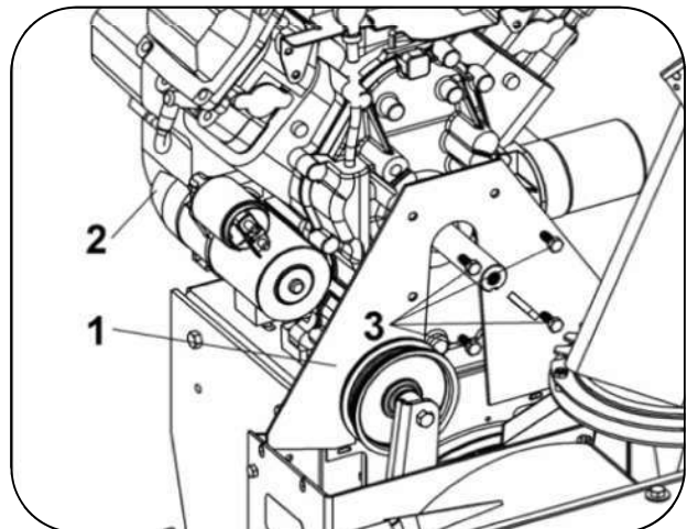
Installing the guard
