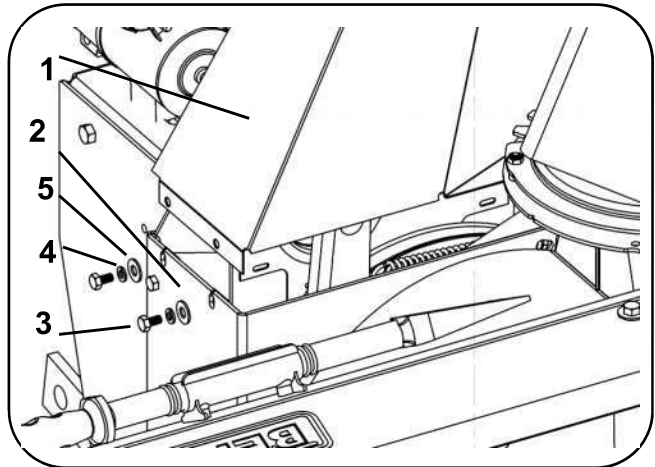
Installing the belt guard
