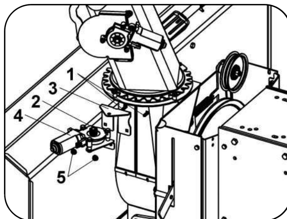
Motor installation
