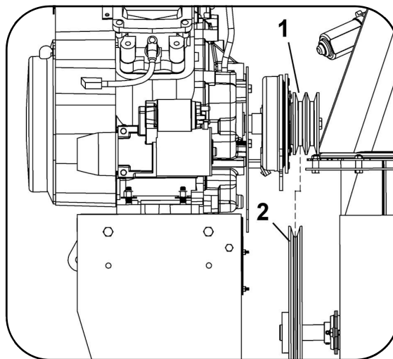
Parallel pulley alignment error
