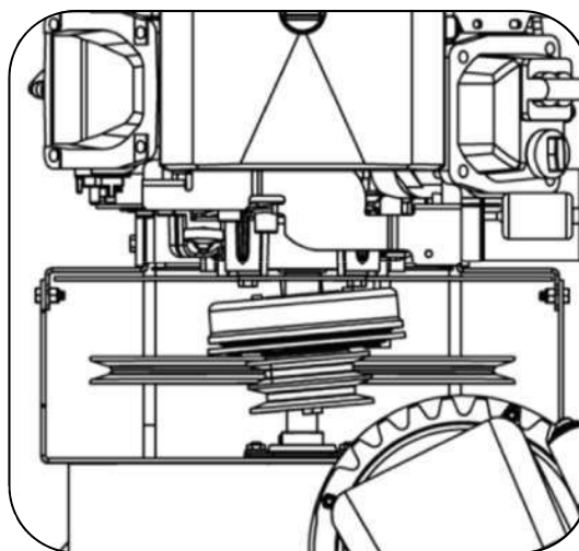
Angular pulley alignment error
